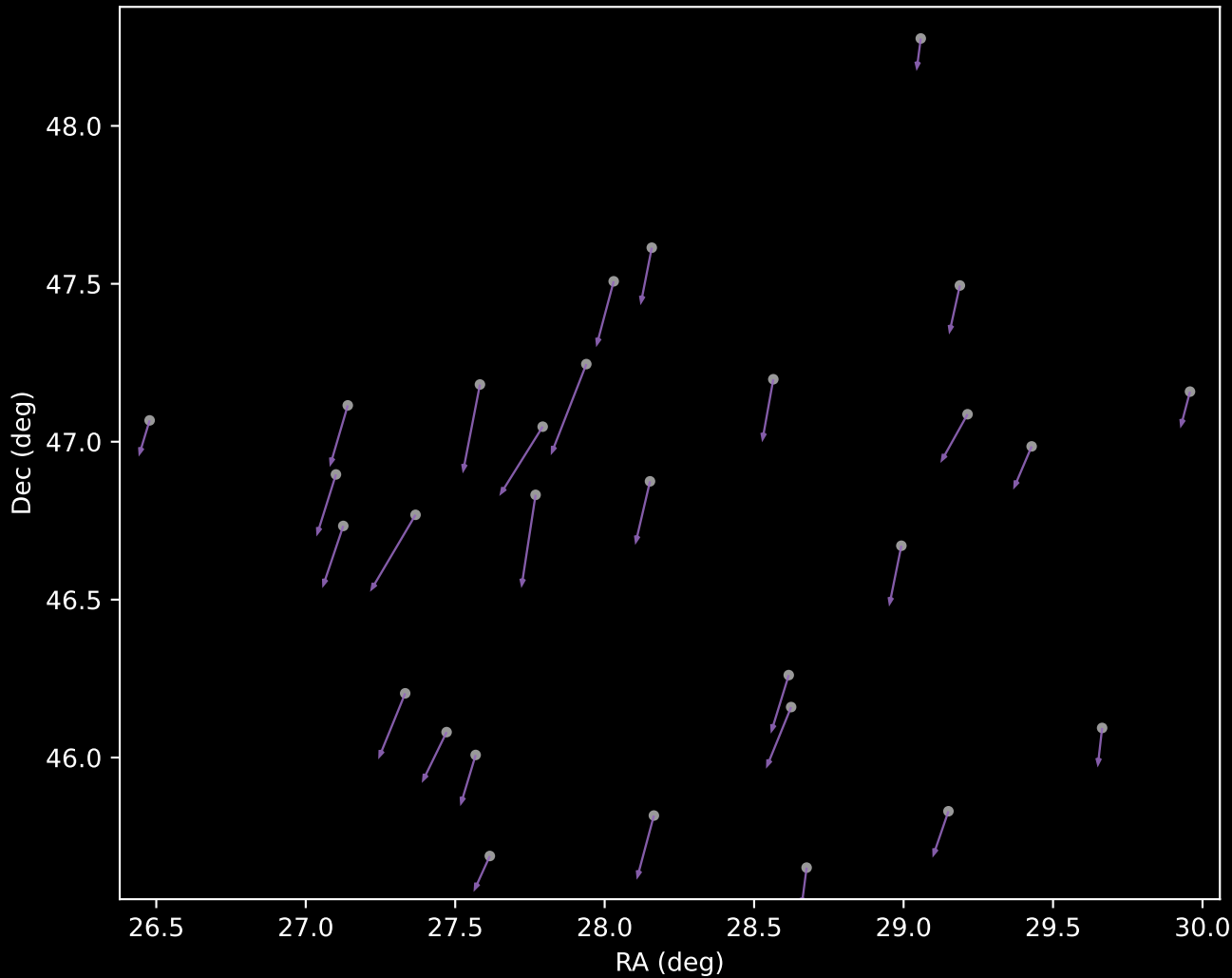
APOGEE DR17 Cluster 8 Proper Motion Vectors (n=29)
