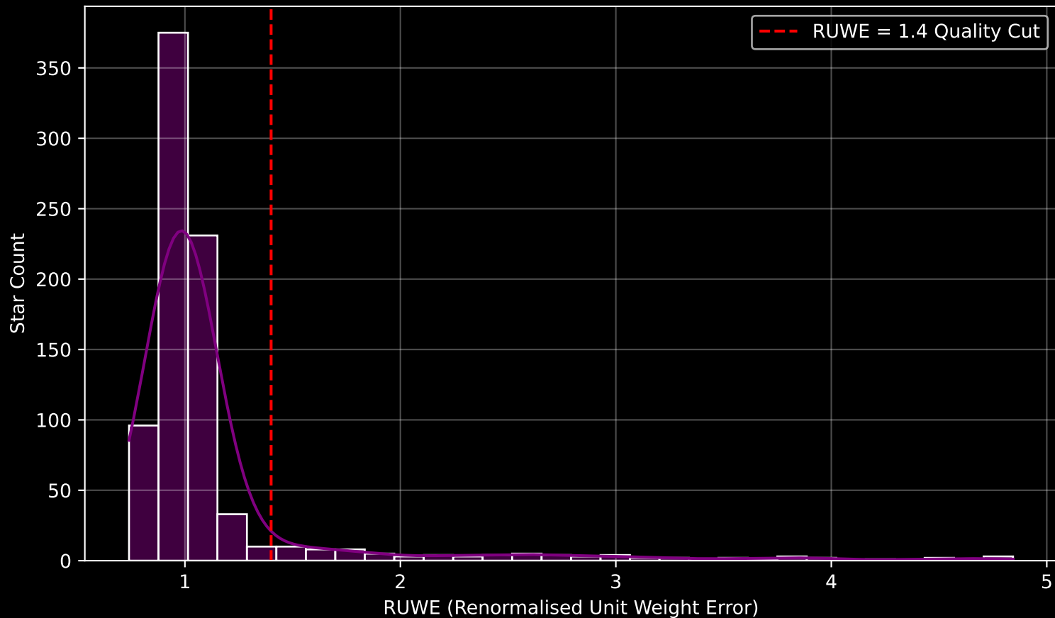
GAPOGEE DR17 Field [K06_078+16] RUWE Distribution (n= 826)
