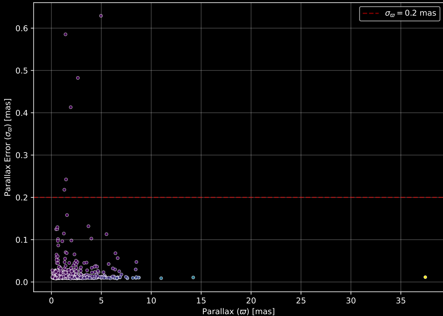
APOGEE DR17 Field: [K06_078+16] Parallax Quality (n= 848)
