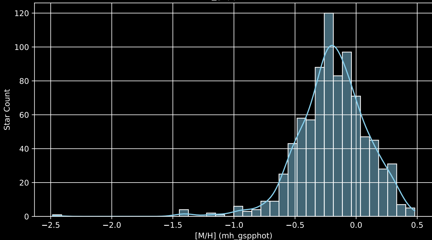
APOGEE DR17 Field: [K06_078+16 [M/H] (mh_gspphot) (n= 844)
