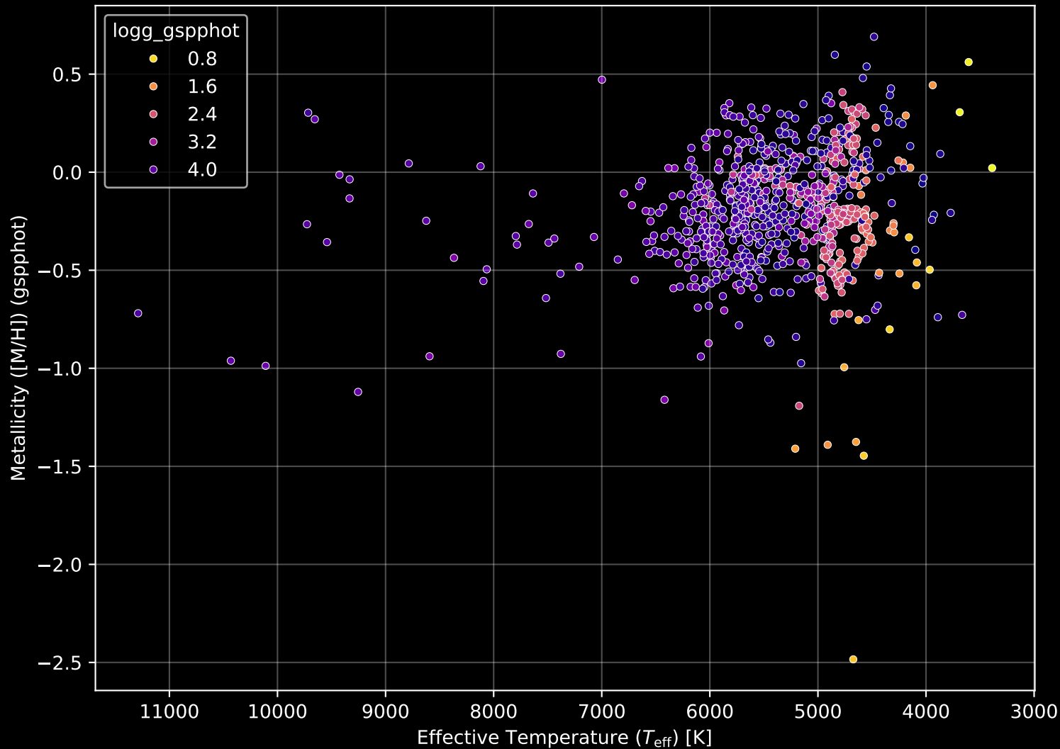
APOGEE DR17 Field: [K06_078+16] Stellar Population Parameters (n= 848)
