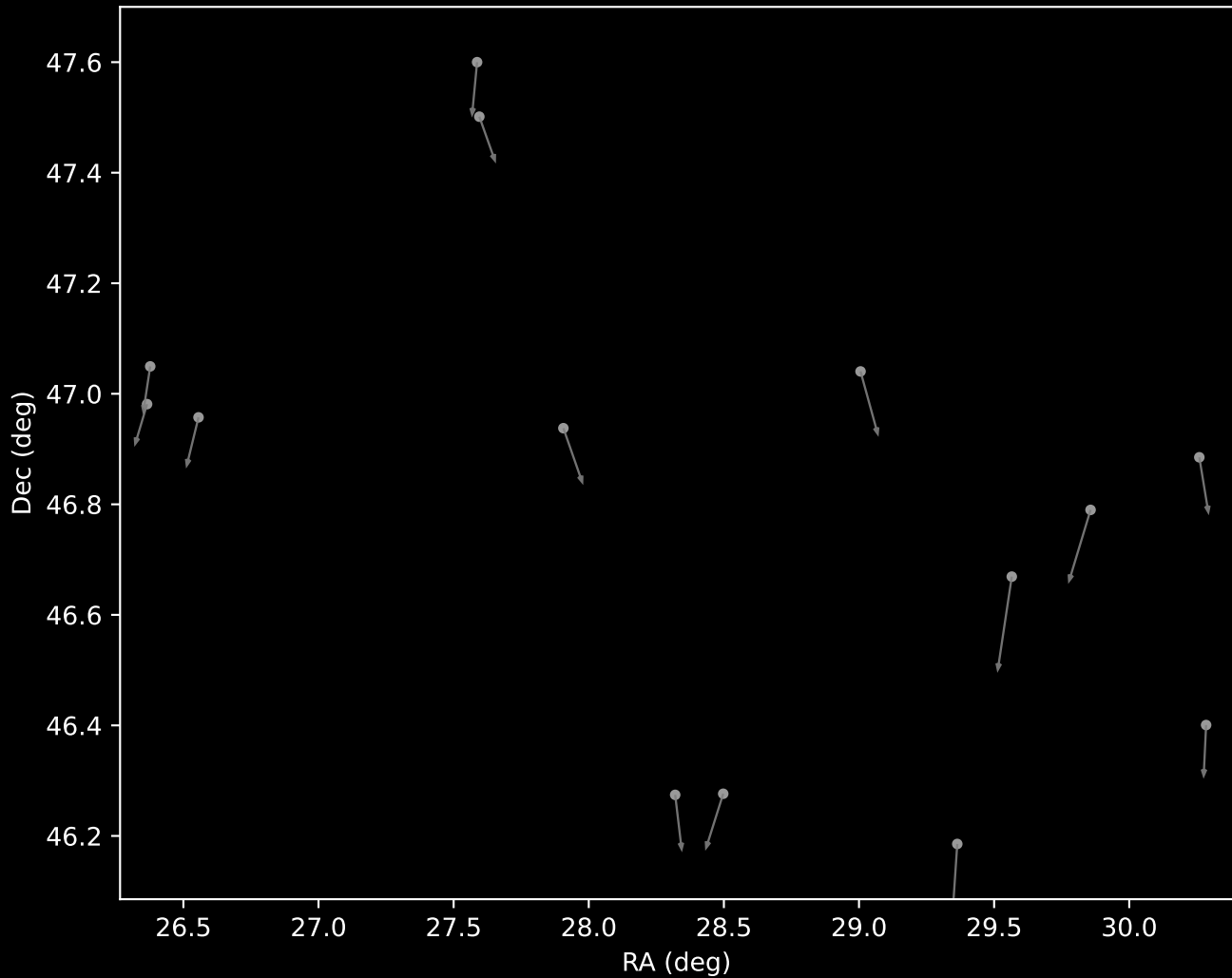
APOGEE DR17 Cluster 34 Proper Motion Vectors (n=14)
