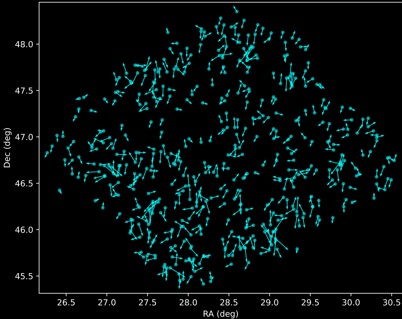
APOGEE DR17 Noise Stream Proper Motion Vectors (n=464)
