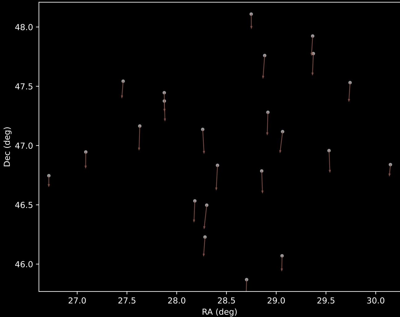
APOGEE DR17 Cluster 30 Proper Motion Vectors (n=23)
