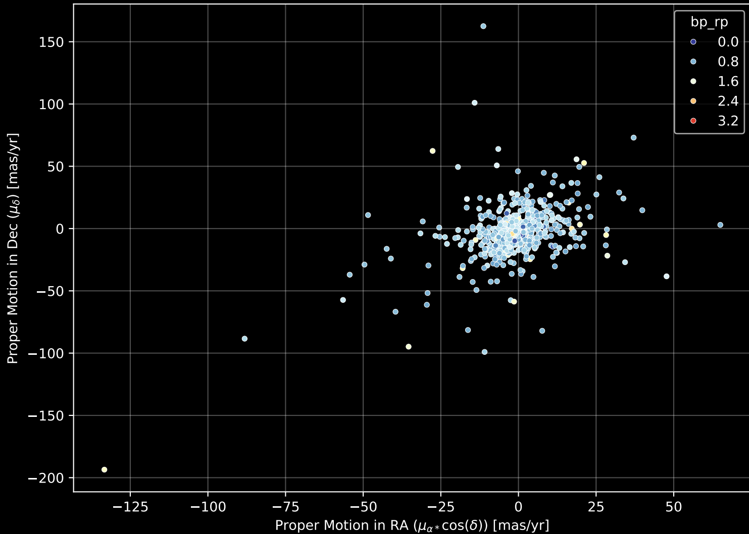
APOGEE DR17 Field: [K06_078+16] Proper Motion Diagram (n= 848)
