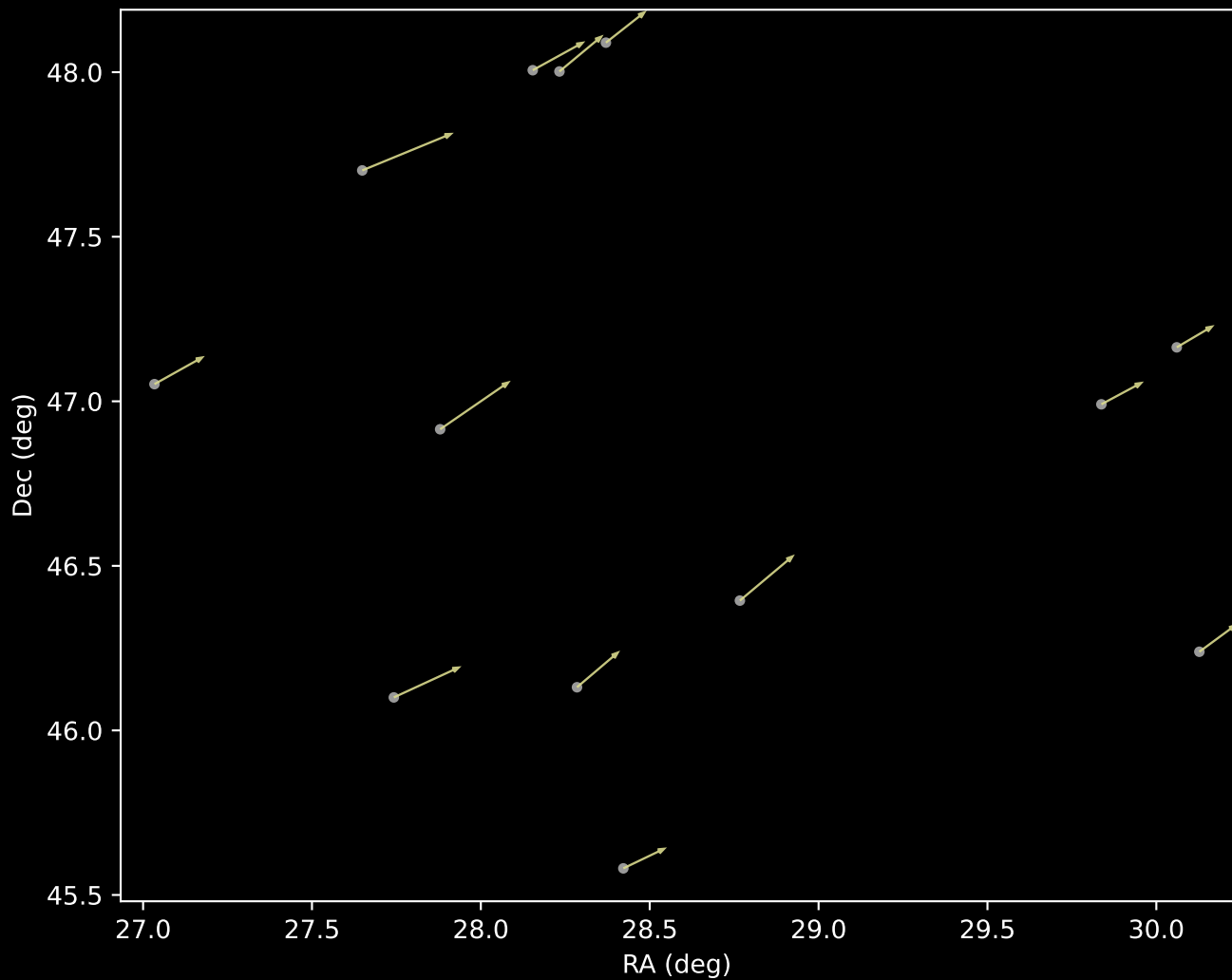
APOGEE DR17 Cluster 17 Proper Motion Vectors (n=13)
