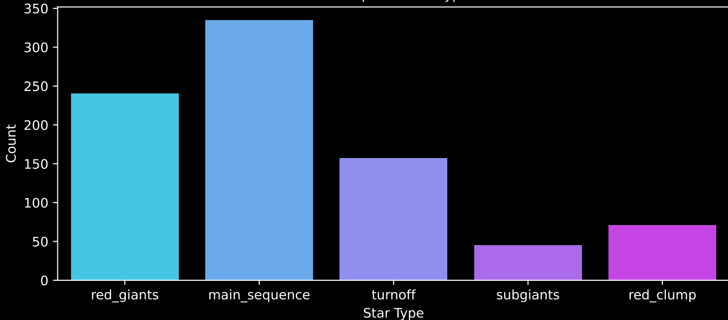
APOGEE DR17 Field: [K06_078+16] Count plot of Star Type
